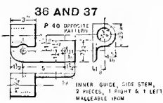
Figs. 1416-1418. Inner Side-stem Guide.
